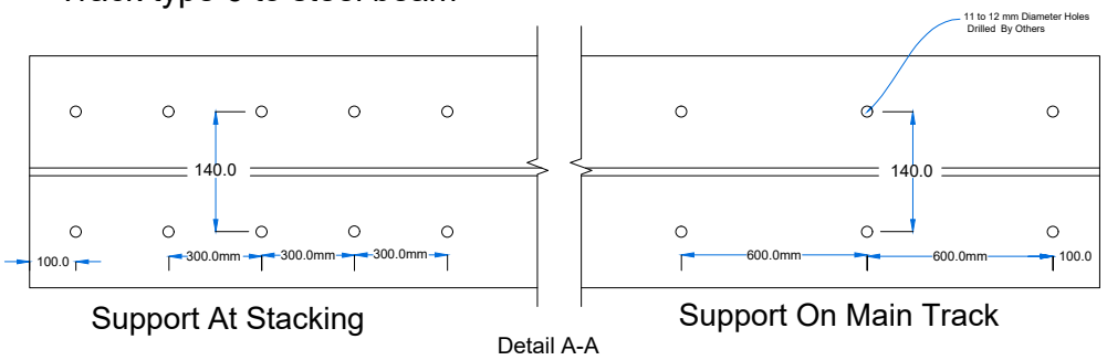
SS1- Track & Support Beam HOLE DRILLING POSITIONS Track type 6
